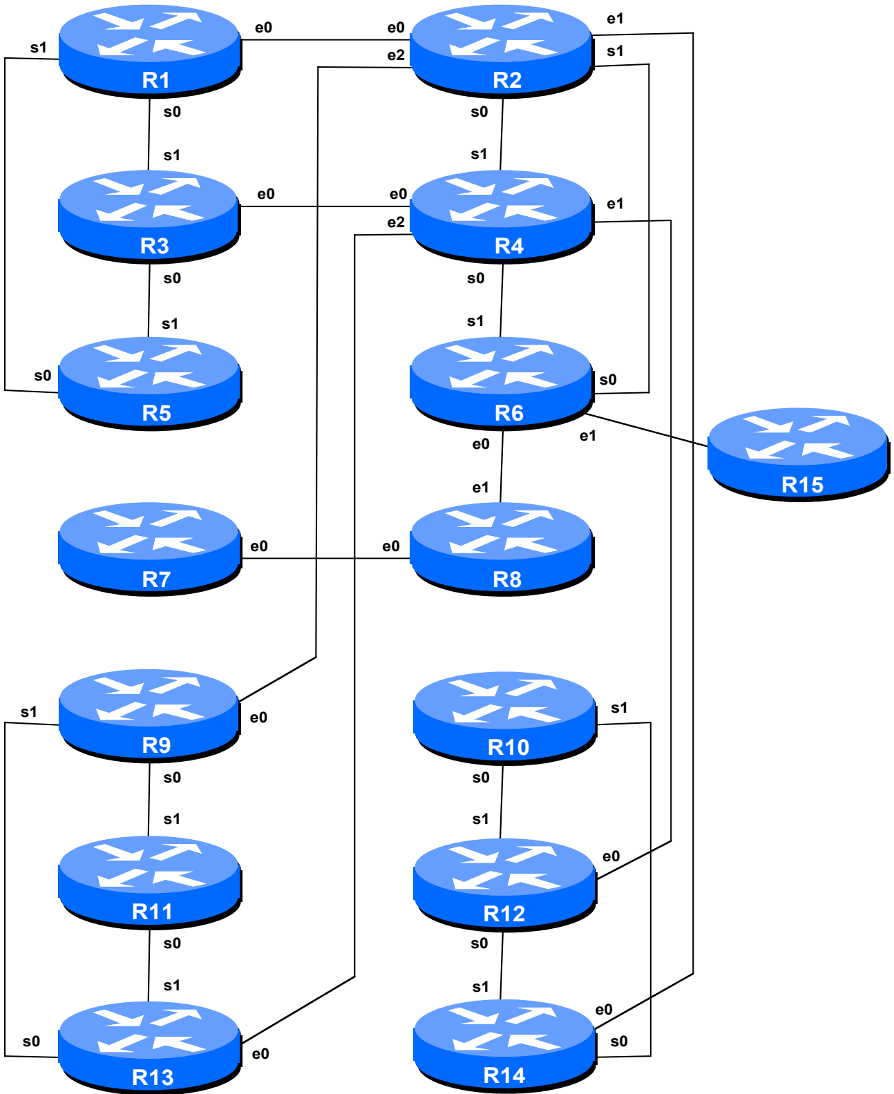
Figure 4 – RFC2270 Lab Physical Layout
